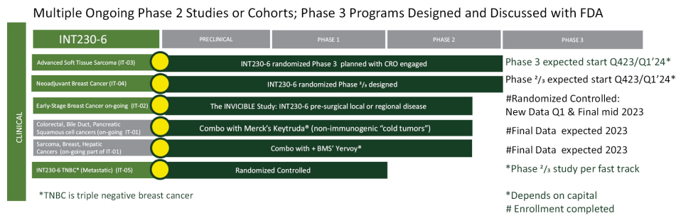
Figure 2 – Pipeline
